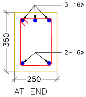
PLINTH BEAM
