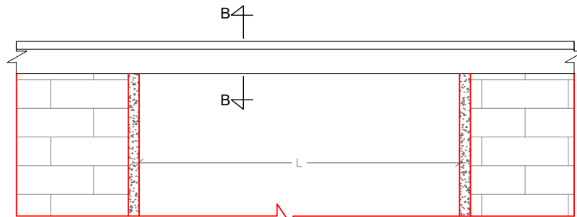
ELEVATION OF EXTERNAL FACE
