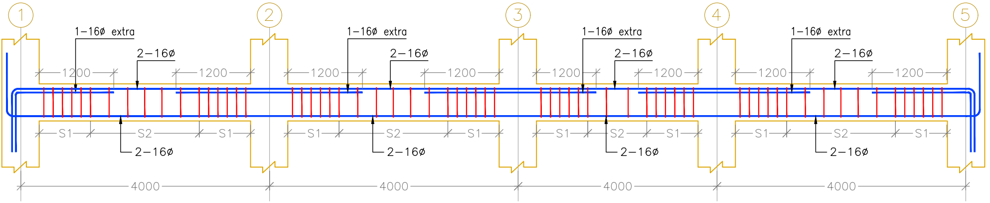
L-SECTION DETAIL OF BEAM ALONG GRID-A & B
