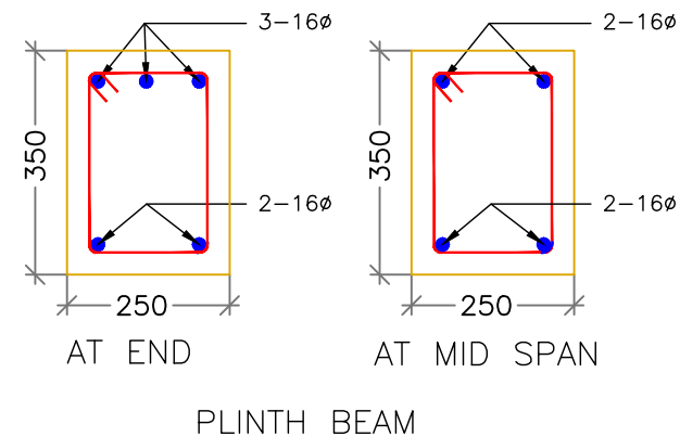
CROSS SECTION DETAILS FOR BEAM
