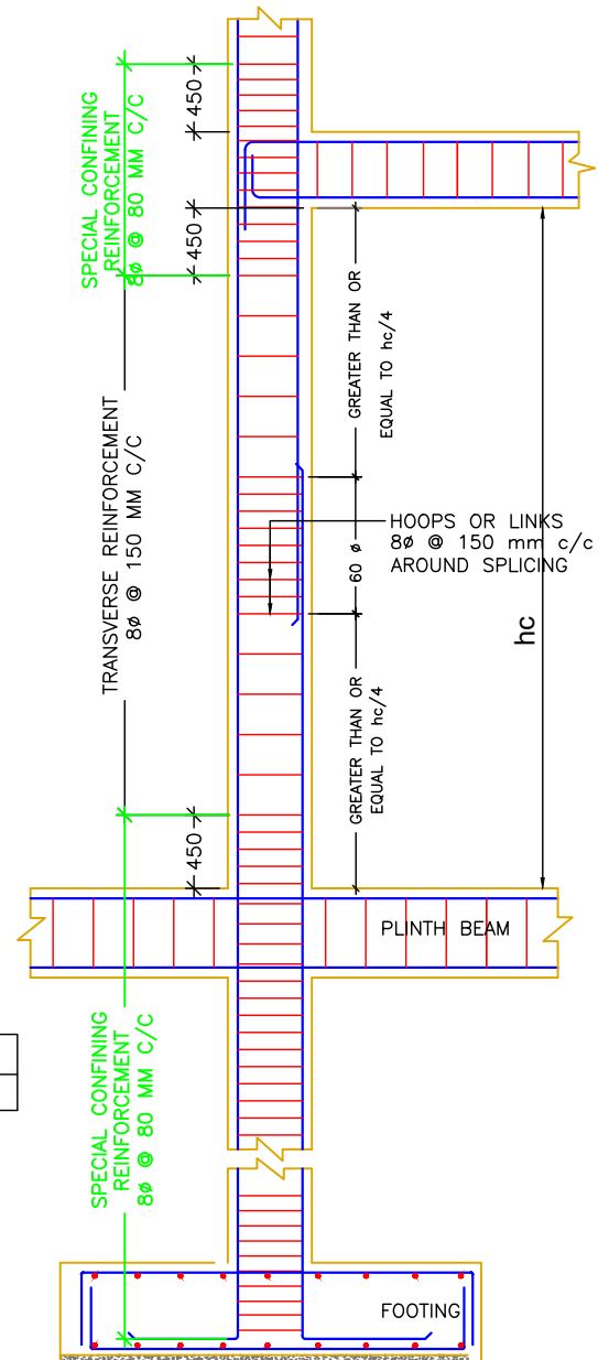
SPLICE WITH OFFSET CRANKED BAR IN COLUMN
