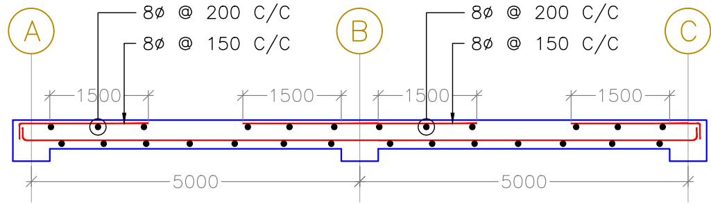
SLAB SECTION AT Y-Y
