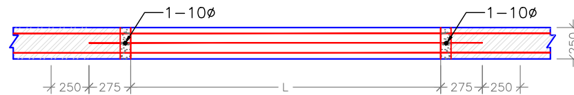
TOP REINFORCEMENT LAYOUT PLAN
