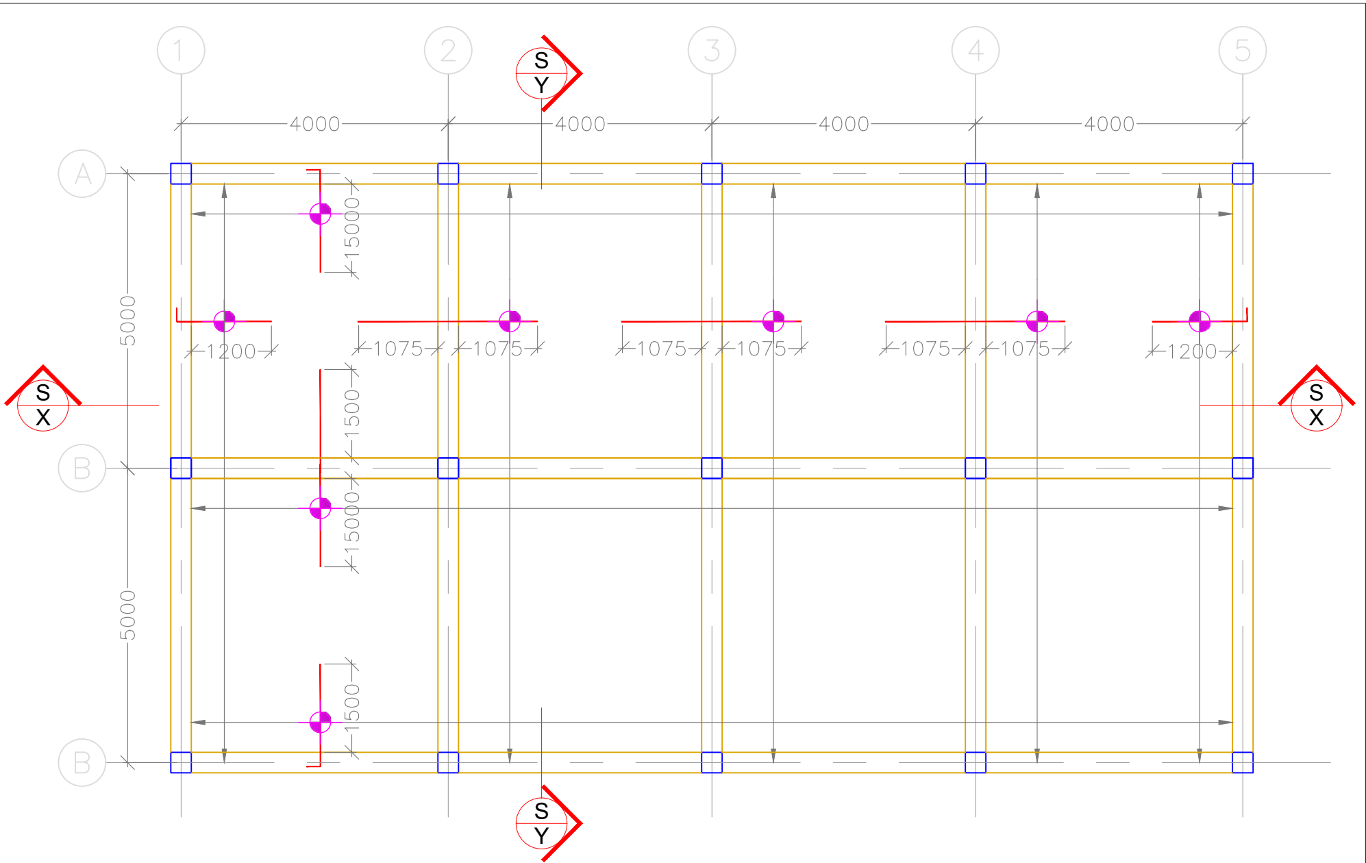
TOP REINFORCEMENT LAYOUT PLAN AT ROOF SLAB
