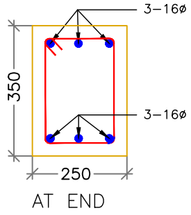
ROOF BEAM
