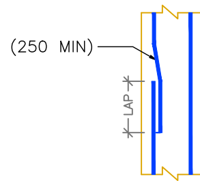
SPLICE WITH OFFSET CRANKED BAR IN COLUMN
