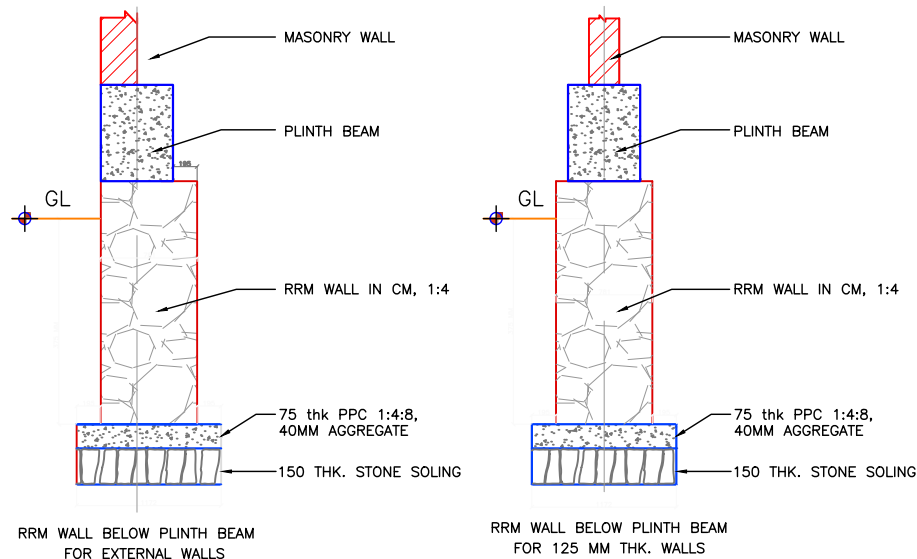
TYPICAL FOUNDATION WALL DETAILS
