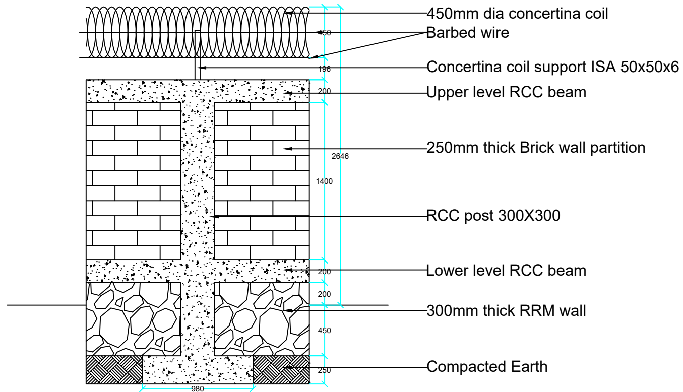
ELEVATION DETAILS
