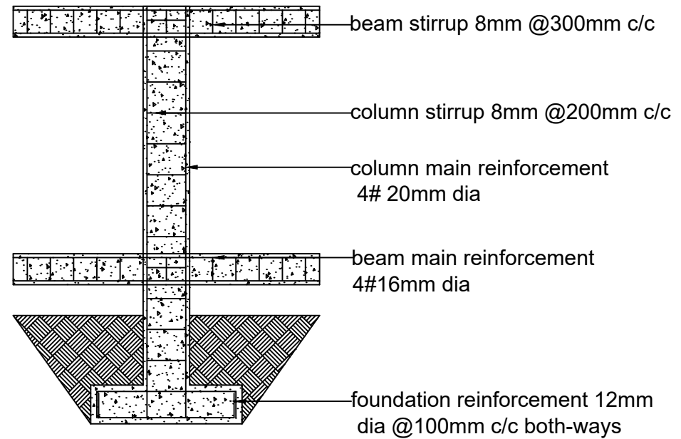
REINFORCEMENT DETAILS
