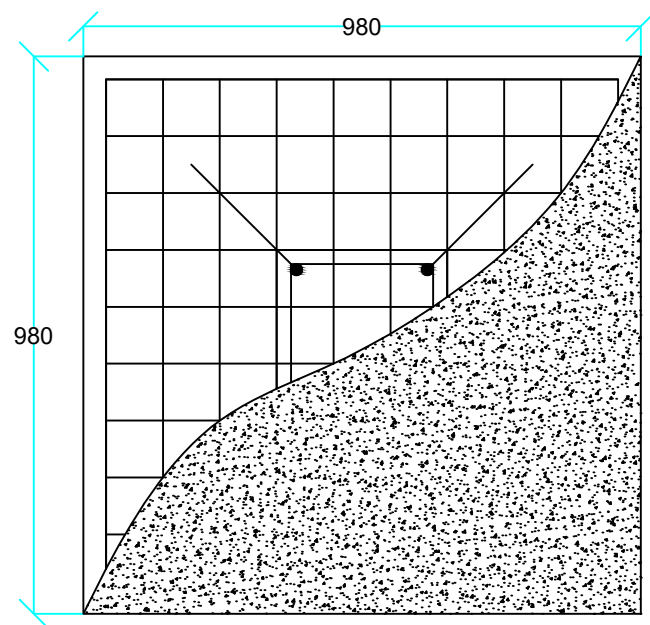
Foundation Pad details
